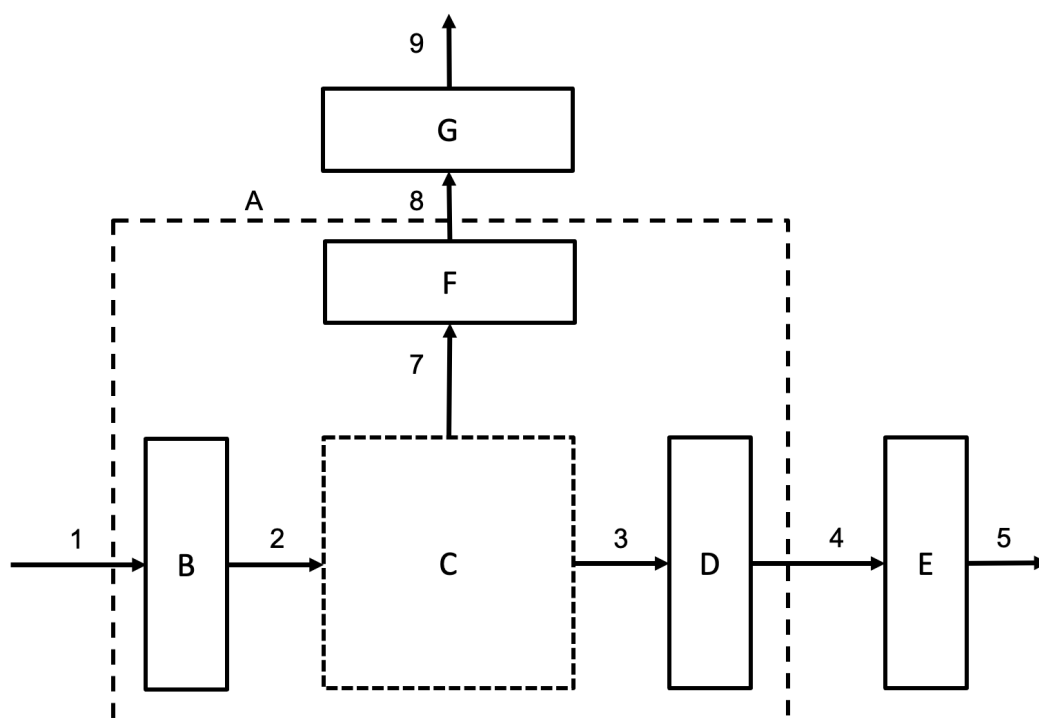
Figure 12 – Balance boundary of the resource exergy analysis for the coverage of a heating and cooling demand by a CHP plant with a heating target temperature above and a cooling target temperature below the reference temperature
