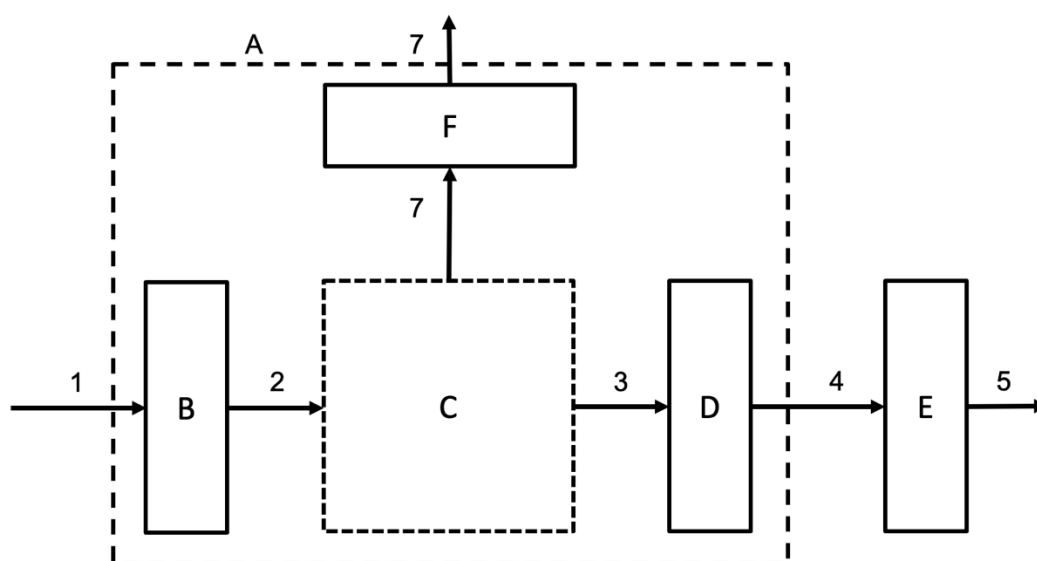
Figure 11 – Balance boundary of the resource exergy analysis for the coverage of a heat demand by cogeneration
